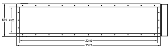
DISCHARGE END
