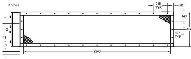
INTAKE END
