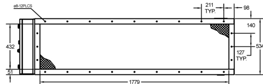
INTAKE END
