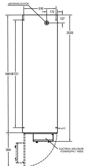
TOP VIEW
