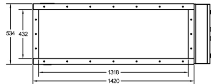
DISCHARGE END
