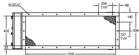
INTAKE END
