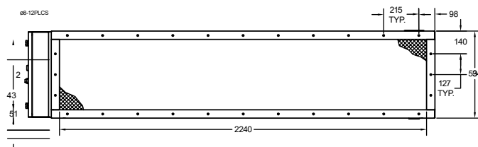
INTAKE END
