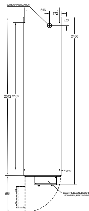
TOP VIEW
